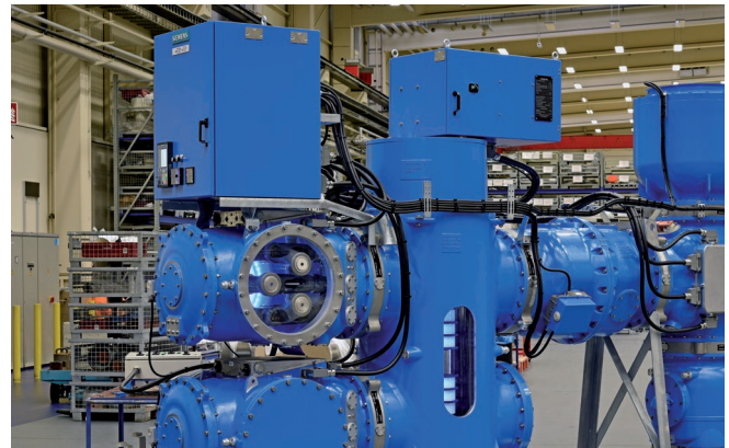
8VN1 Blue GIS® switchgear with vacuum interrupting technology and clean air insulation
