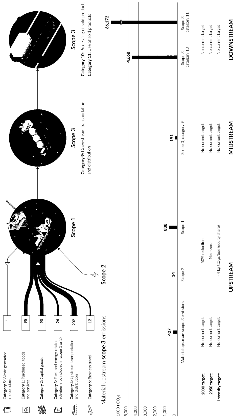
Figure 11: Operational control GHG emissions across the value chain (in 1000 t CO 2 e)
