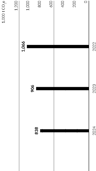
Figure 17: Operational control scope 1 GHG emissions
