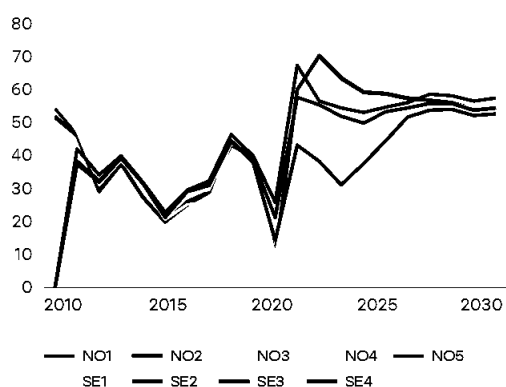
Area Prices in the base scenario 2021-2030, incl. historical prices 2010-2020 EUR/MWh (real 2021)
