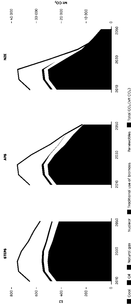
Figure 5: Total primary energy supply by fuel and scenario
