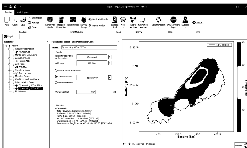
Figure 4: EMU (EMU utilities) software by EMGS with new functionality for rock physics modeling and quantitative interpretation of CSEM inversion results in terms of reservoir properties.
