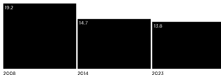
Average containership fleet speed (knots)
