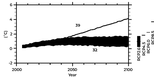
Global average surface temperature change (relative in 1986-2005)
