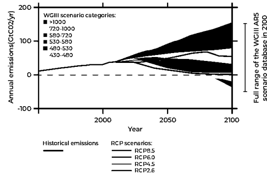
Annual anthropogenic CO 2 emissions
