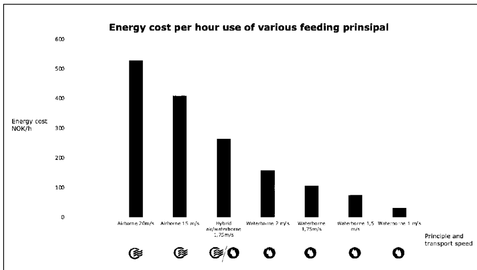
Figure 19 - Energy cost per hour by use of various feeding principles. Source: AKVA group
