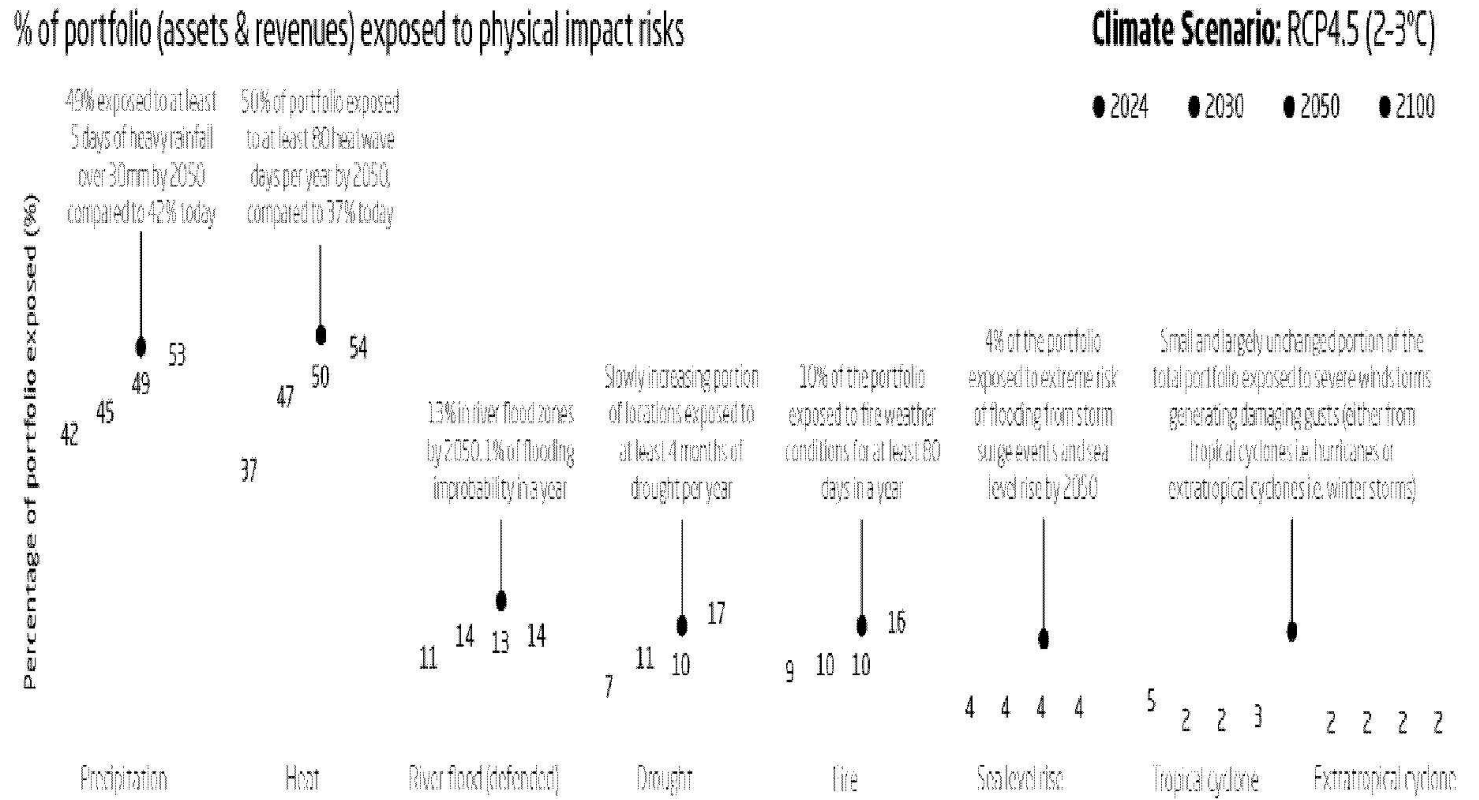
Figure 1: Physical risk exposure under an RCP4.5 scenario:
