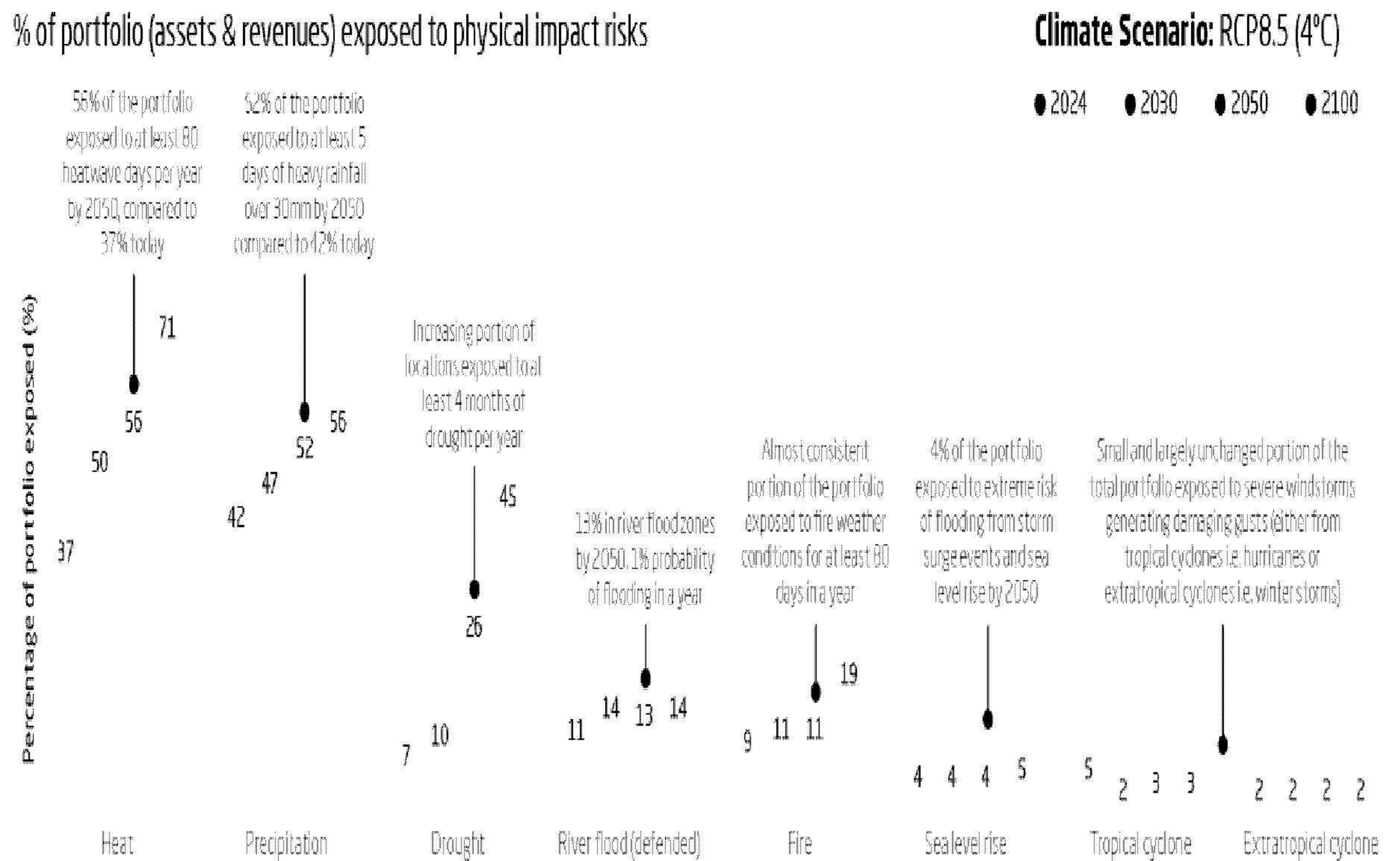
Figure 2: Physical risk exposure under an RCP8.5 scenario:
